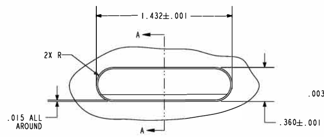
HOLE DETAIL
